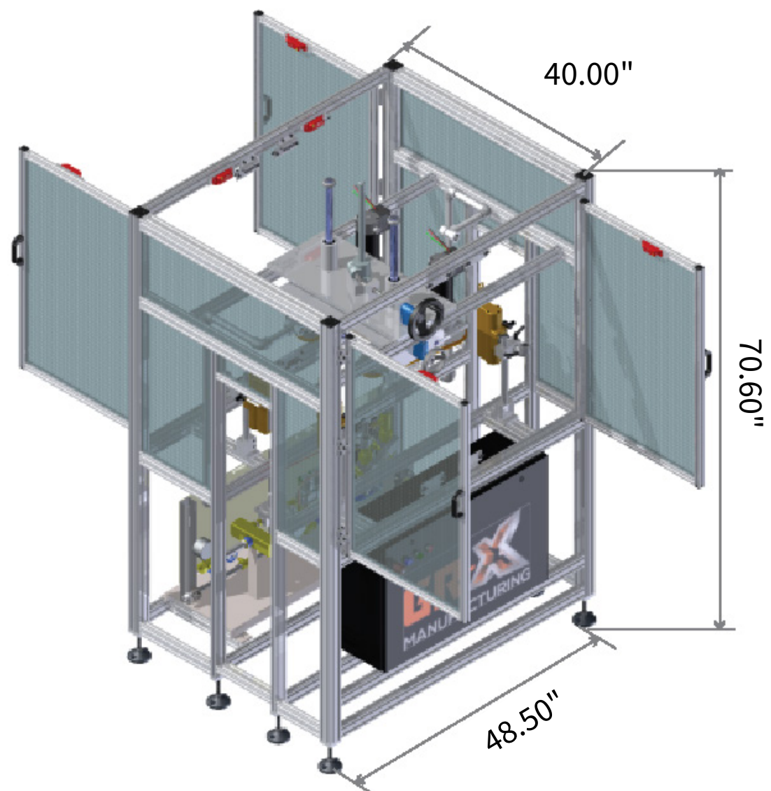
Four Burner Dimensions
