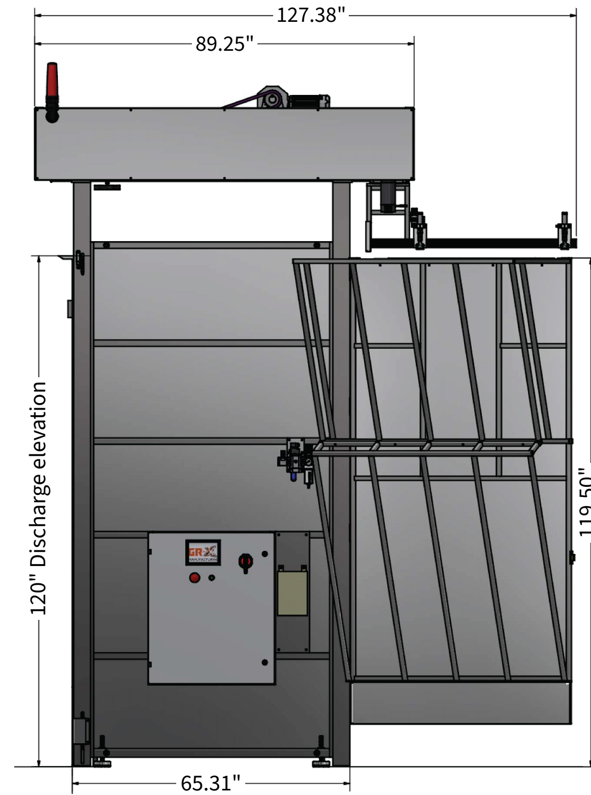
SIDE VIEW
